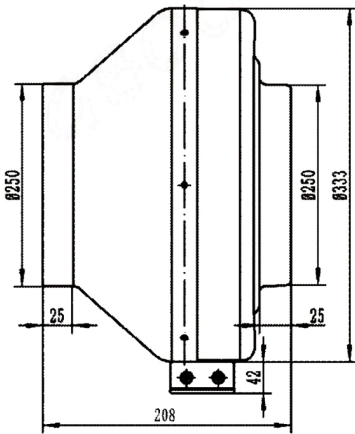
★ Dimensions Drawing(外观图)
